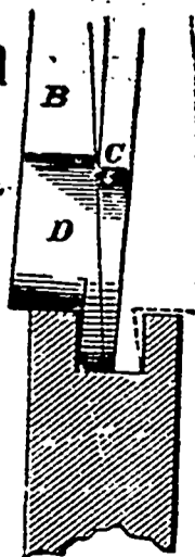
FIG. 2—CUTTER NEARLY USED UP.
