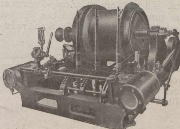
ELECTRIC HOISTS made with either one or two drums, and any required diameter of Drum up to 48". Your choice of seven sizes, from ten to fifty horse power. Over a quarter of a century of successful manu- facturing of Mine Hoists.
