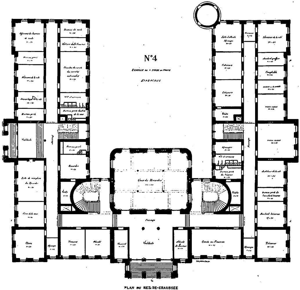
FIRST PREMIATED DESIGN QUEBEC CITY HALL COMPETITION.
