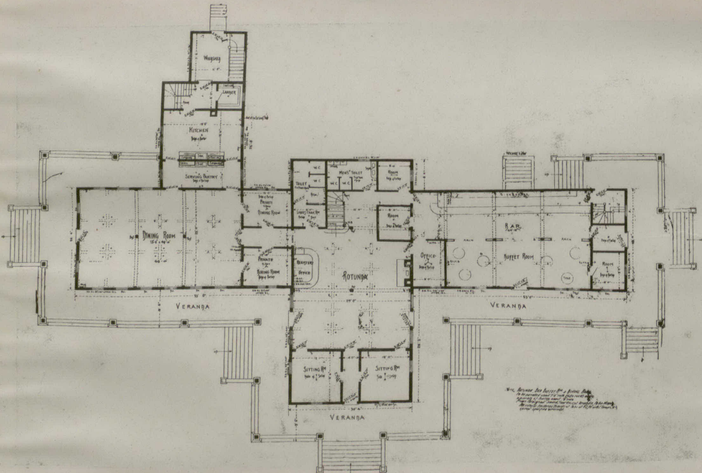
— GROUND FLOOR PLAN — SCALE 8 FT. = 1 IN.
