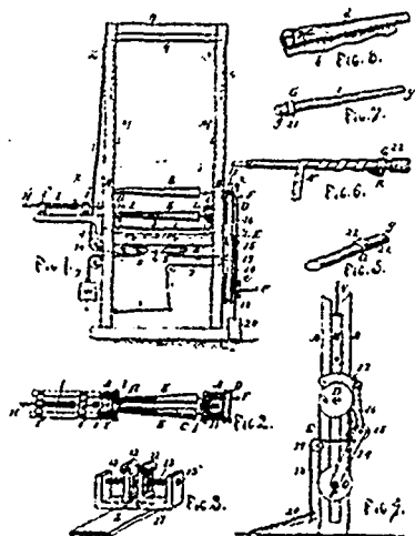
29390 Sherwood's Veneering Machine.
