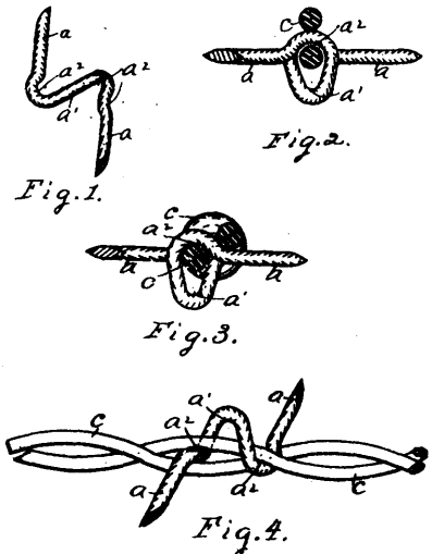
16171 Bralnard's Improvements on Wire Barbs for Fences.
