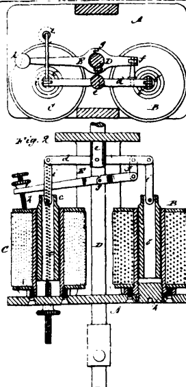
16170 Parker's Improvements on Electric Lamps.
