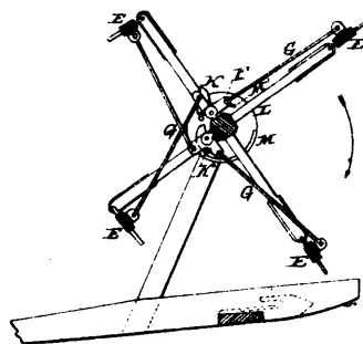
12792 Akens' Improvements on Harvester Reels.
