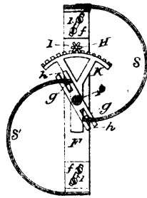
12783 Wales' Improvements on Mechanical Thermometers.
