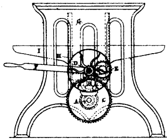
12786 Cowan & Ballantine's Improvements on Planing Machines.
