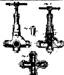
10887 Gear's Improvements on Valves.
