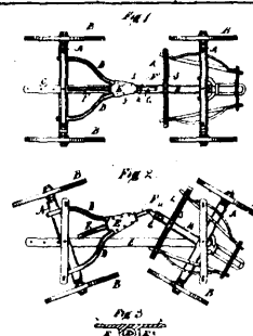
10884 Shaw &amp; Cook's Improvements on Waggon Gears.
