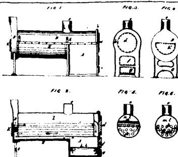
10890 Hall &amp; Lane's Improvement in Portable Boilers.
