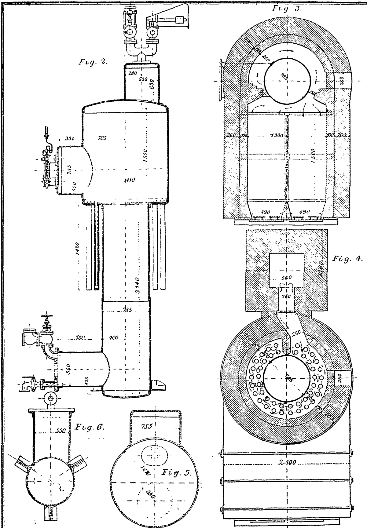
BERGMANN'S HIGH-PRESSURE BOILER AT THE VIENNA EXHIBITION.
