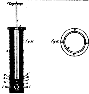
10193 Morin's Key for Water Cocks.
