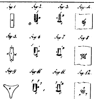
10502 D'Aubigne's Improvements on Tubular Rivets.
