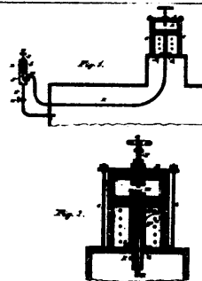
7321 Sovell's Improvements on Safety Valves.
