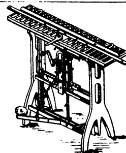
7315 Carter &amp; Stewart's Improvements on Mortising Machines.
