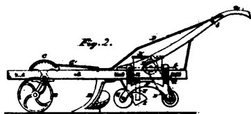
7308 Rowe's Combined Horse Hoe and Seed Drill.
