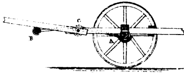
5706 McCarter's Waggon Tongue Support.
