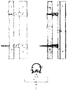
5703 Linklater's Improvements in Conductor Pipes and Holdfasts.
