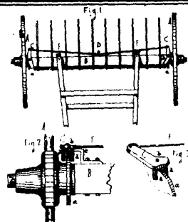
6120 Sharp's Improvement on Horse Rakes.
