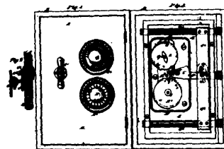
6125 McCaskey's Combination Lock.
