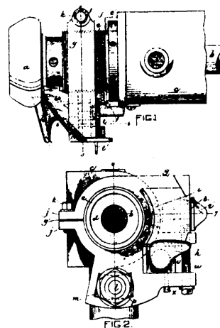
40135 Fuller and Plummer's Heel Trimming Machine.
