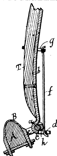
21000 Baker's Thill Coupling.
