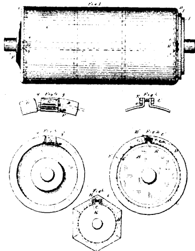
20999 Smith's Device for Tightening Bolting Cloth.
