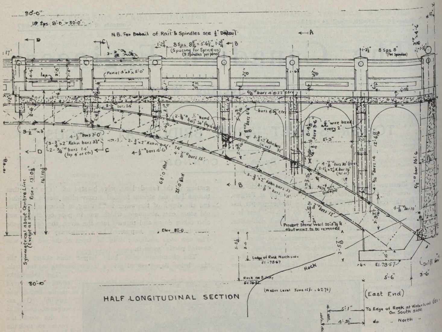
DESIGN FOR 80-FT. x 25-FT. CONCRETE ARCH BRIDGE OVER GRAND RIVER AT FERGUS, ONT.
