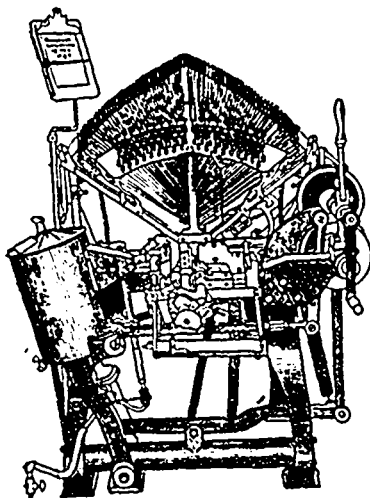
Rogers Typograph Line-casting Machine
