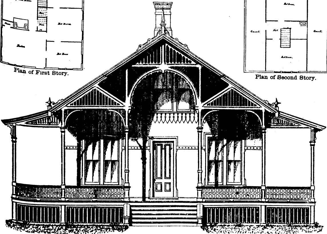
DESIGN FOR COTTAGE, COSTING $1,200.—FRONT ELEVATION.
