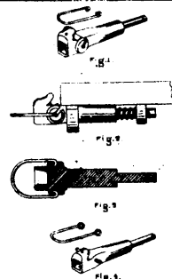
9881 Crackett's Improvements on Draw-bars.
