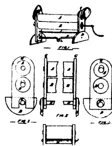
9888 Kinleyside & Wilson's Improvements on Clothes Wringers.
