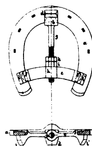
9878 Bigg's Improvements on Horse Shoes.
