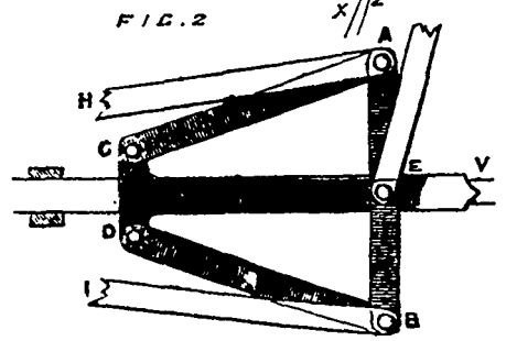
A SUBSTITUTE FOR LINK MOTIONS. (See page 239 )
