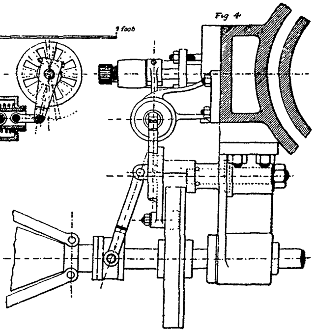
DETAILS OF HORIZONTAL ENGINE AT VIENNA. (For description, see page 287.)
