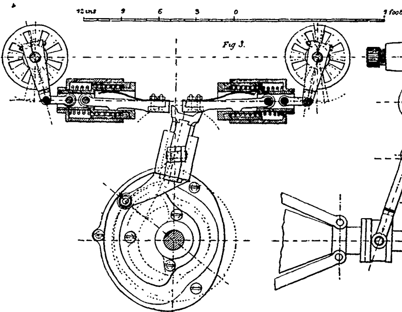
DETAILS OF HORIZONTAL ENGINE AT VIENNA. (For description, see page 287.)
