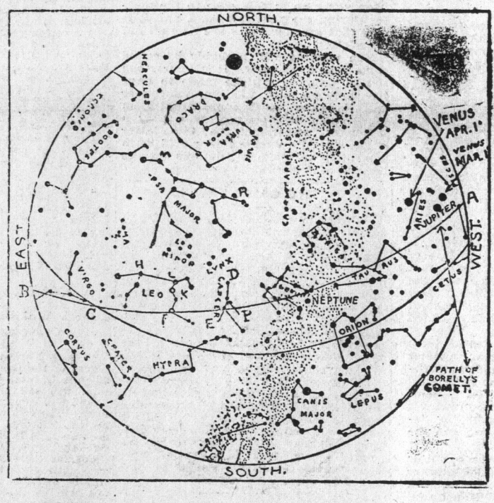
Fig. 1—Constellations March 1.
