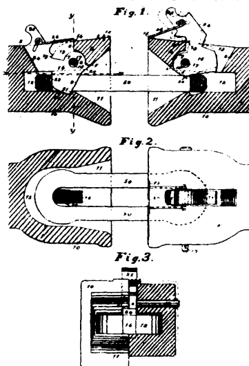
26928 Chisholm's Car Coupling.
