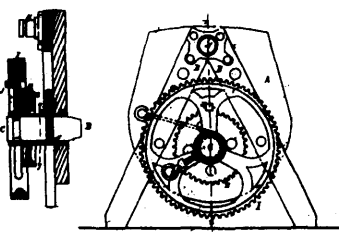
3268 Lewis' Improvement on Churn Powers.
