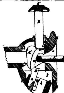
3266 Lamb &amp; Avery's Self-acting Car-coupler.
