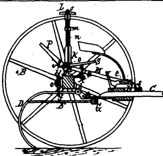
3265 Sweet's Plaster Sower.
