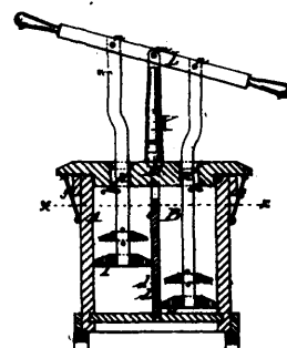
3269 Mathias &amp; Coons' Improvements in Churns.
