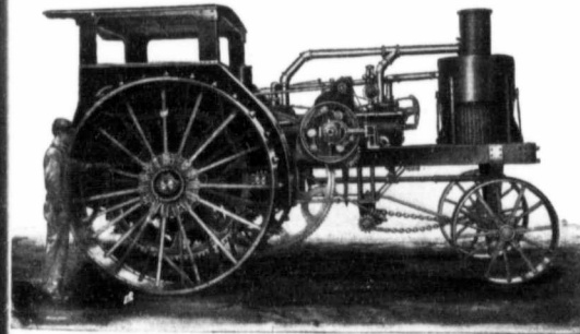
Avery Gas or Oil Tractor Five Sizes: 8-16, 12-25, 20-35, 25-50 or 40-80 H. P.
