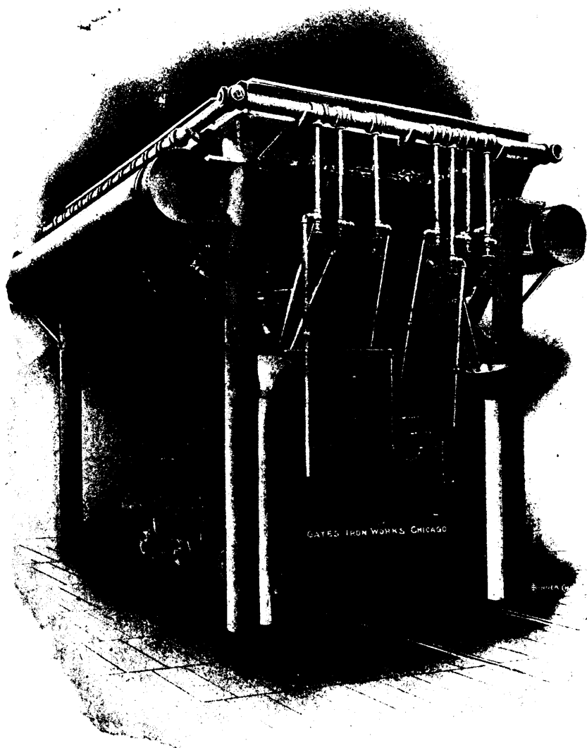
RECTANGULAR WATER-JACKETED COPPER FURNACE. Size, 44 in. x 160 in.
