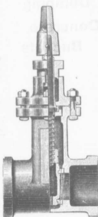
Sluice Valve
