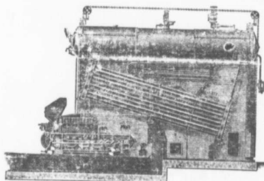
"B. & W." PATENT WATER TUBE BOILER. HEATER AND IMPROVED MECHANICAL STOKER.
