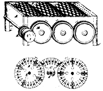
12457 Doten's Improvements on Rotary Fire Grates.
