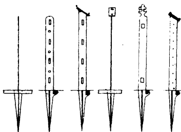
2556 May &amp; Pettit's Cast Metal Fence Post.
