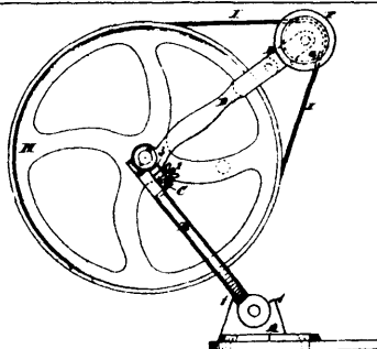
2554 Emerson &amp; Sabin's Harvester Grinder.
