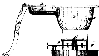
2559 Chase's Coal Oil Cooking Stove.
