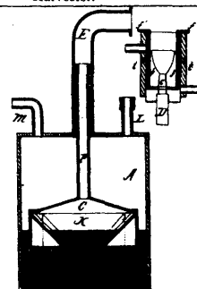
2555 Dayton &amp; Jones' Machine for Carburetting Air.
