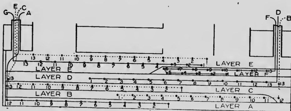
Fig. 8. Diagram showing arrangement of thermometers in forward hold, those on starboard side being indicated by continuous lines and those on port side by dotted lines.
