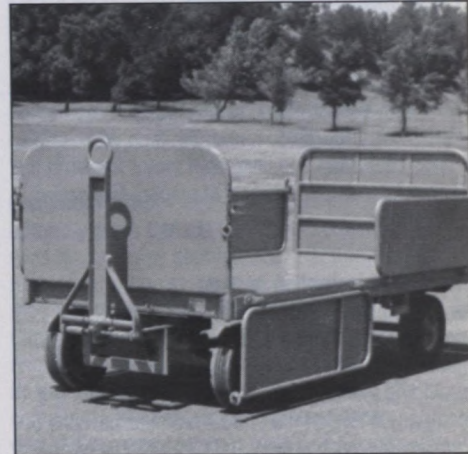
Model 322-6119 baggage/cargo trailer
