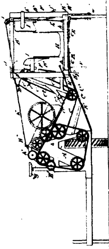
42762 Connell's Grain Shocking Machine.
