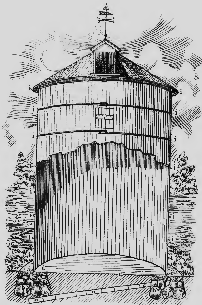
FIG. 5. Longitudinal section of Stave Silo, showing: a a , drain; b , foundation; c , ground floor; d , cement floor inside; e , cement floor outside; i i , etc., hoops.
