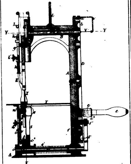
26521 Wileman's Sewing Machine.
