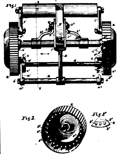
26517 Hanika & Rogers' Lawn Mower.
