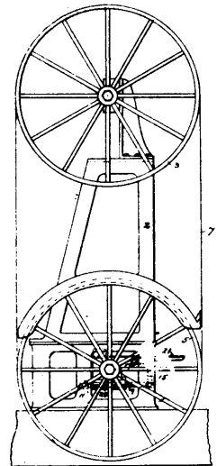
26514 Esplin's Wheel for Regulating the Tension of Band Saws.
