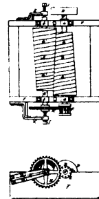
13289 Brown's Improvements in Grinding Mills.
