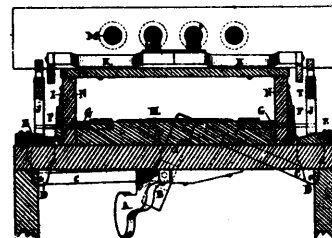
7695 Kydd's Improvements in Organ Stop Actions.
