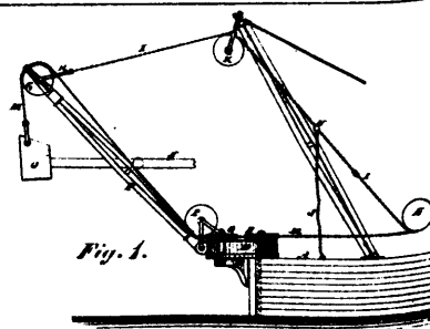
7701 Osgood's Improvement in Dredging and Derrick Machines.
