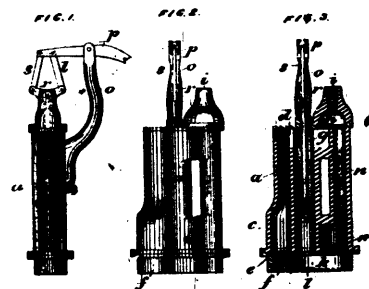
7689 Scott's Improvements on Force Pumps and Fire Engines.
