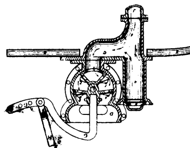
5557 Johnson's Improvements in the "Eureka Pump."
