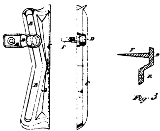
5545 Gillmore's Improvements on Sash-holders.
