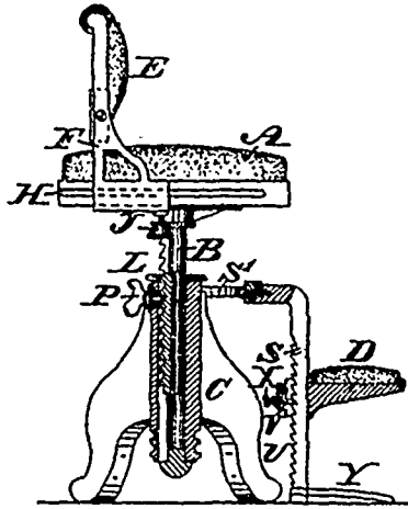
24226 Hayne's Stool for Planos, etc.
