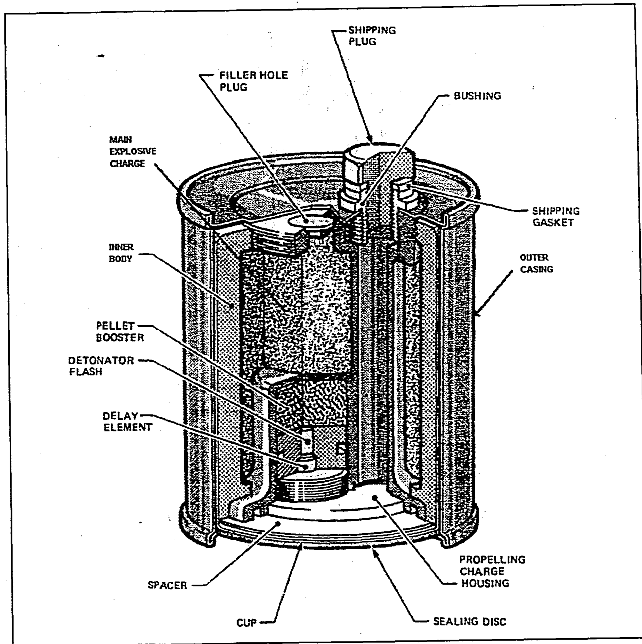
FIGURE 9 - ANTI-PERSONNEL MINE M16A2 SHOWN WITHOUT FUSE, M605
