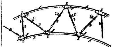
2877 Peck's Machine for Moulding the Frame Work of Vessels, Ships, &c.
