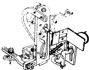
2668 Hansen & Harley's Button Holes and Embroidery Worker for Sewing Machines.
