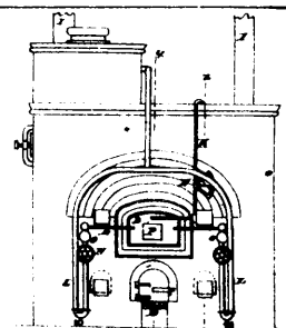
2679 Scowden's Furnace for Converting Iron into Steel.
