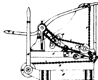
2682 Rodgers' Improvement on Saw Mill Head Blocks.
