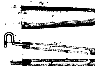
2670 McLeod, Newton & Gladman's Tuyere.
