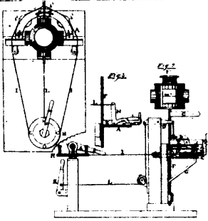
6995 Golden's Improvements in Railway Switches.
