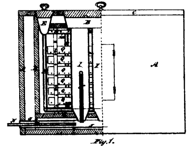
4466 Tozel & Southwood's Freezing Apparatus.
