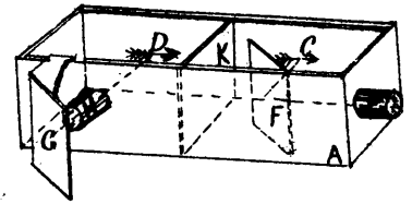
4463 Harris' Reflecting Stereoscopic Camera.
