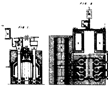
4459 Spice's Gas Apparatus.
