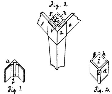
4469 Cleaveland's Joint for Furniture.
