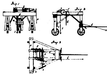
4465 Ayres' Stump Machine.
