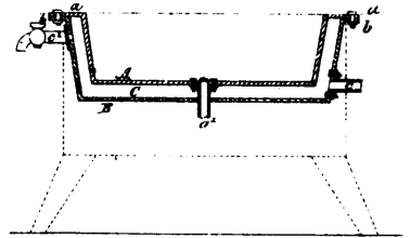
4460 Laubach's Water Cooler.
