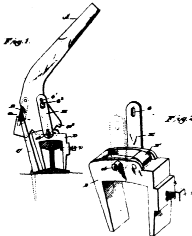
34084 West's Spike Extractor.
