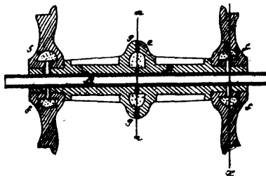
1393 Miltimore &amp; Doty's Car-Axles and Wheels.
