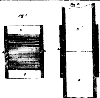
2002 Shay's Pipe-Coupling.
