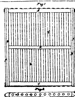
2007 Duffe &amp; Tilton's Gas Purifier Screen.
