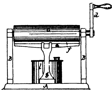
1395 Weston's Machine for Burnishing Photographic Card-Board, etc.
