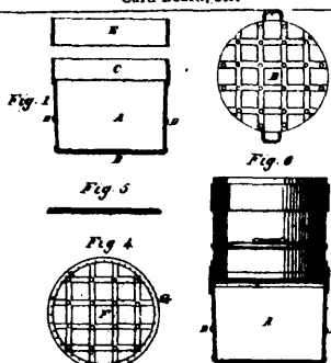
1399 Fraser's Cheese Hoop.
