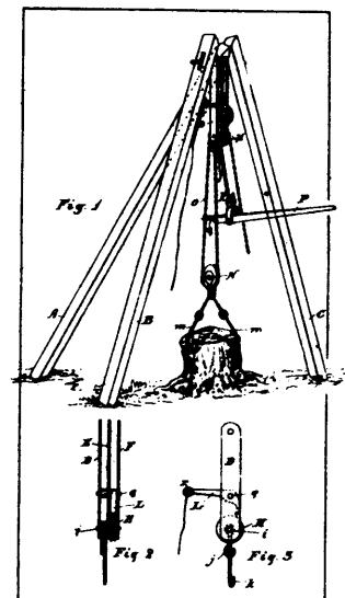
28088 Laframboise's Lifting Machine.
