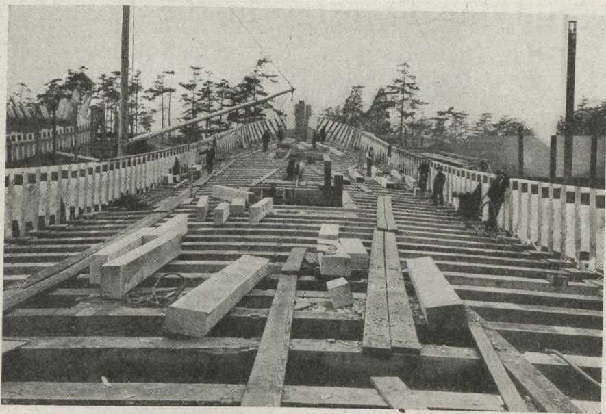
Shipbuilding in British Columbia.—Deck view of a wooden schooner during construction.
