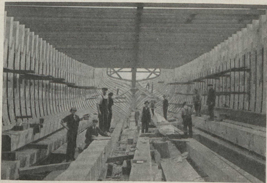
Shipbuilding in British Columbia.—Looking through the skeleton of one of Canada's new feet of wooden freighters on the Pacific Coast.
