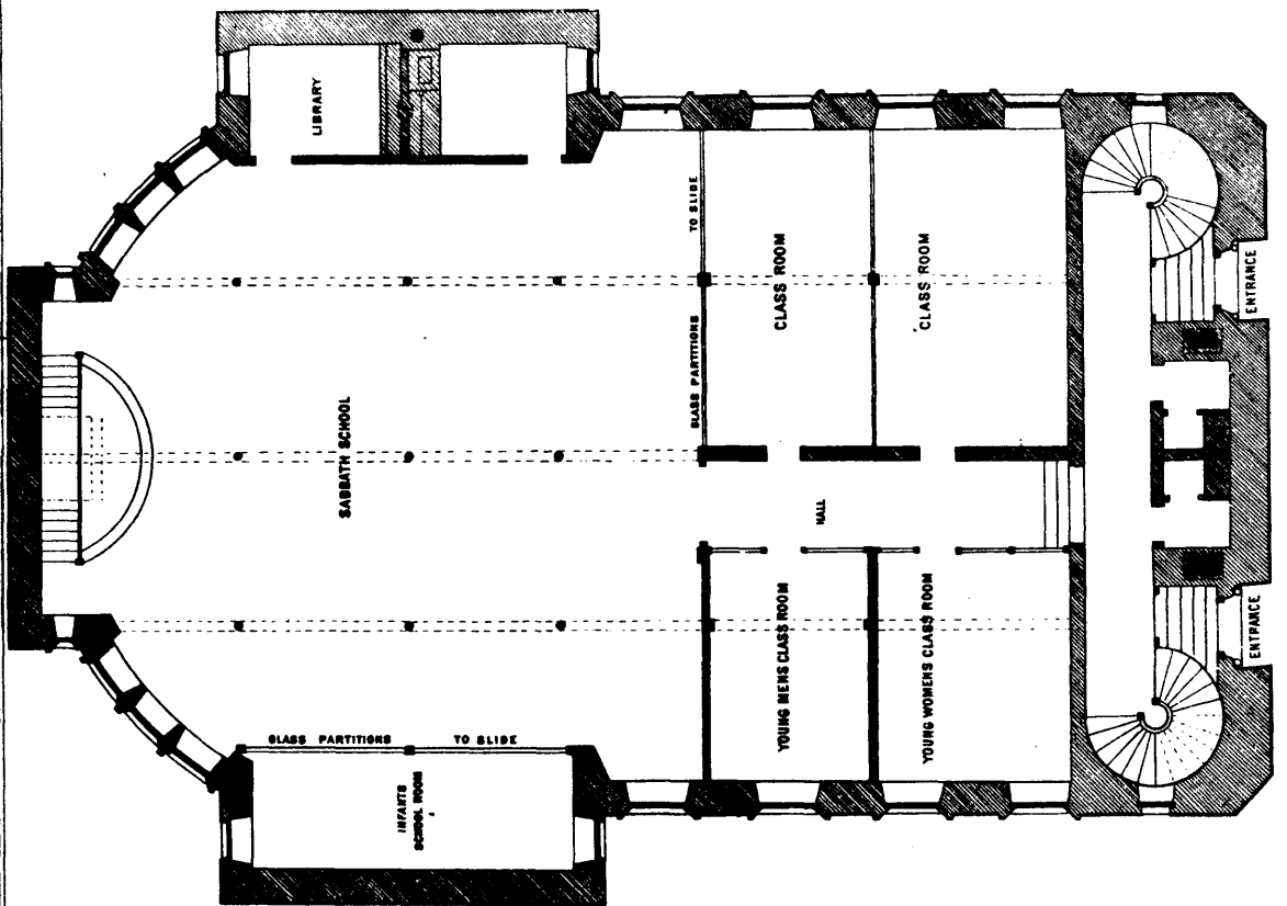
BASEMENT PLAN.
