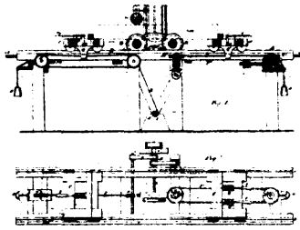
8673 McGuire's Improvements on Saw-mill Carriages.
