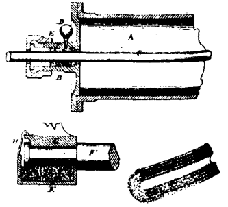
8677 Stewart & Wells' Improvements on Piston Packing.
