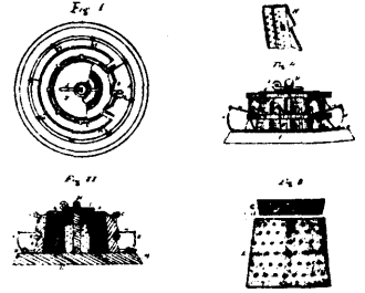
8674 Hubbard's Process for Making Pails from Pulp.
