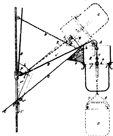
40444 Abbott's Apparatus for Loading and Unloading Vessels
