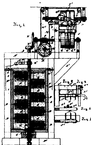
40445 Pfanne's Apparatus for making Varnish.
